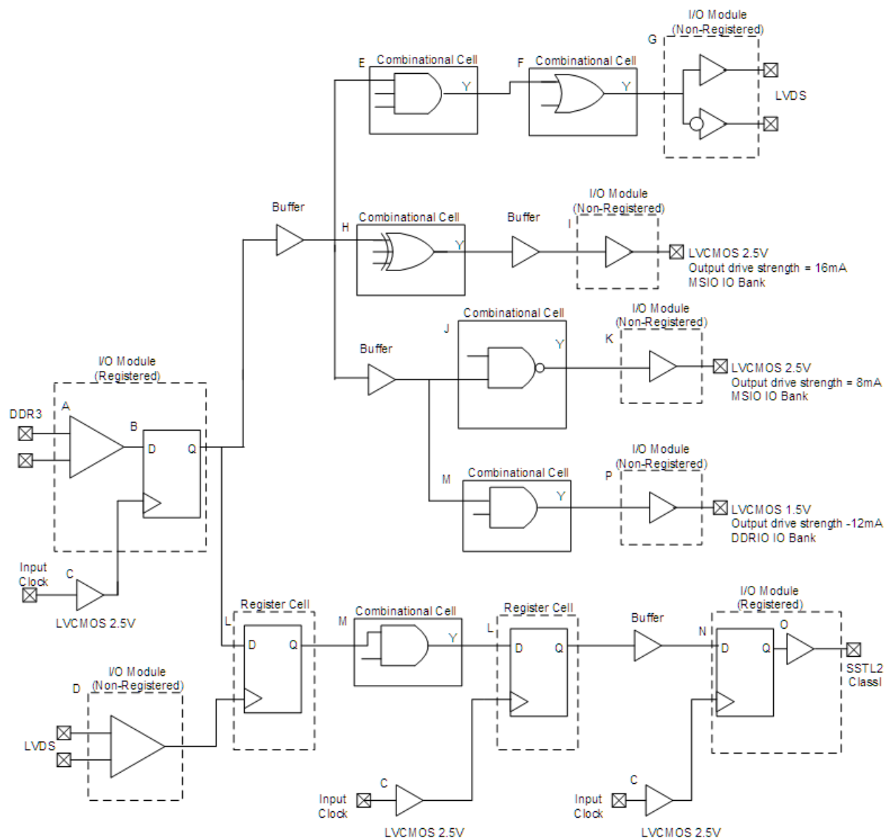
Figure 1 • Timing Model
