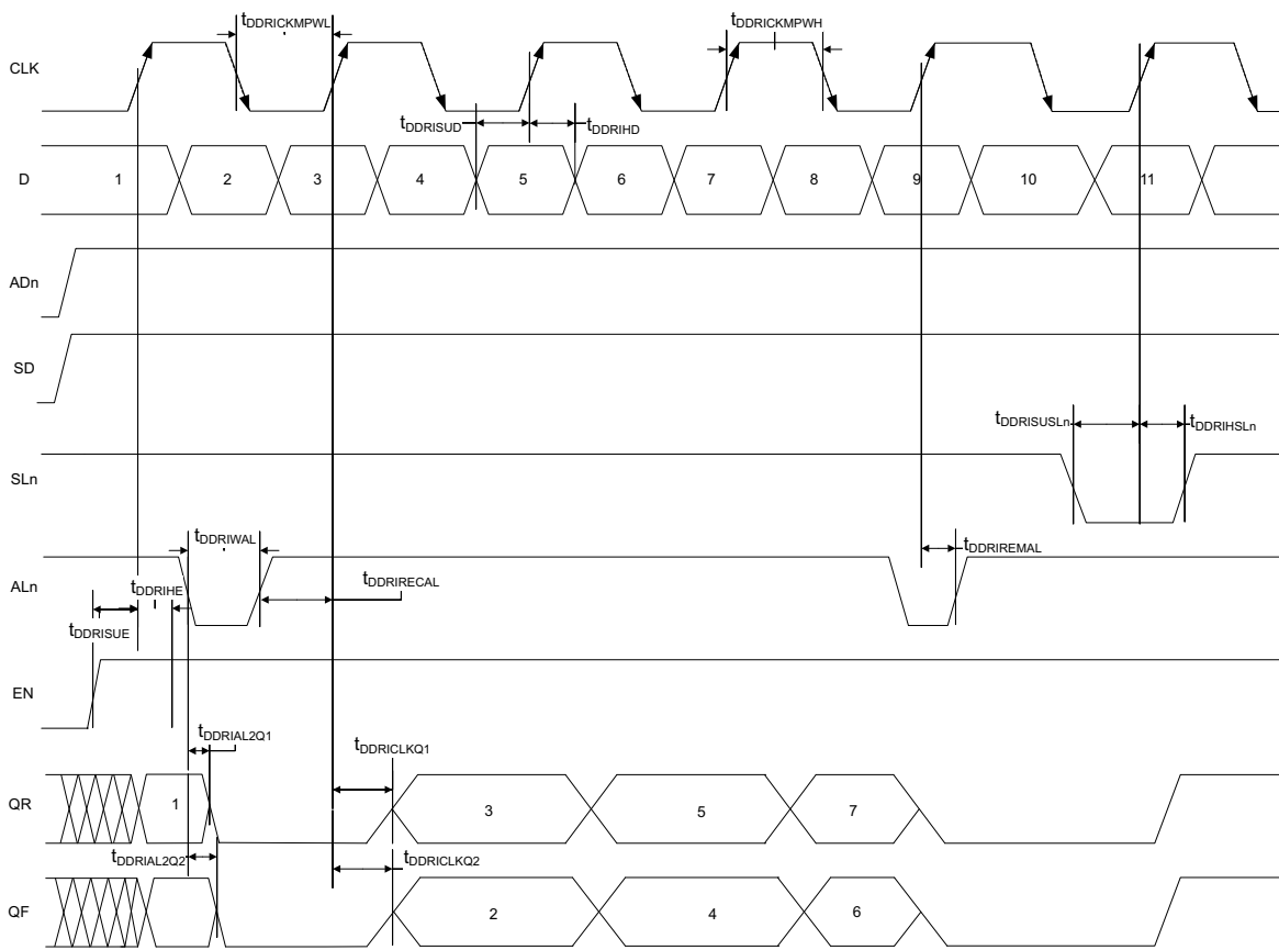
Figure 10 • Input DDR Timing Diagram
