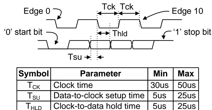
Figure 10. PS/2 Timing Diagram.
