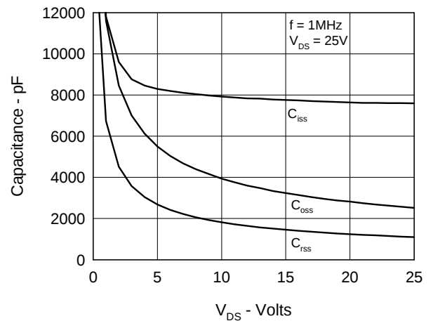
Fig.8 Capacitance Curves
