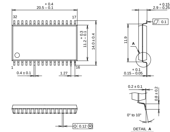
32PIN SOP (PLASTIC) 525mil
