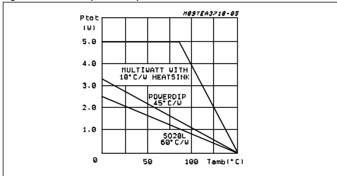
Figure 5. Maximum power dissipation
