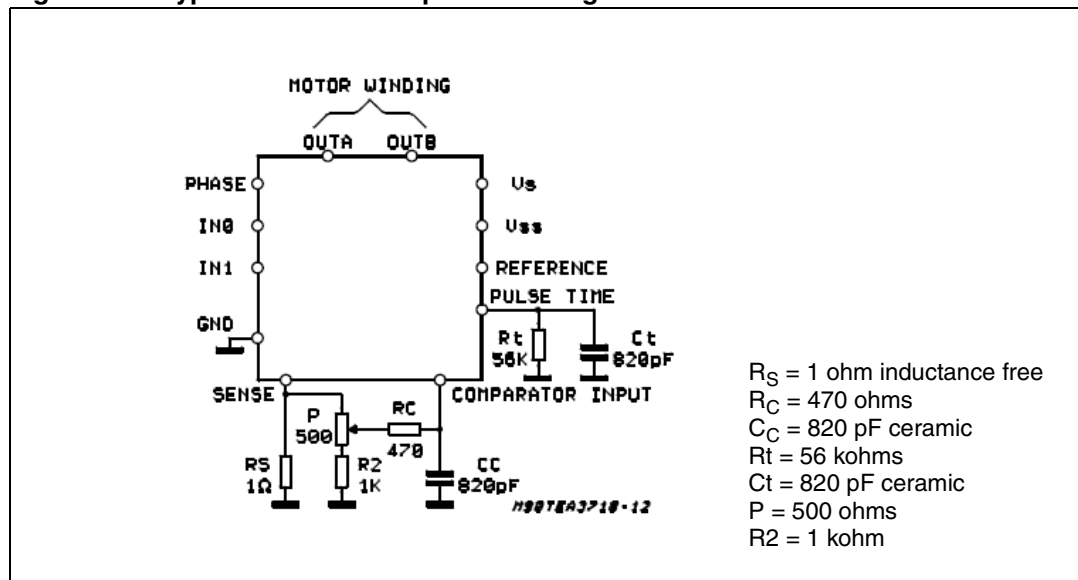
Figure 6. Typical external component configuration
