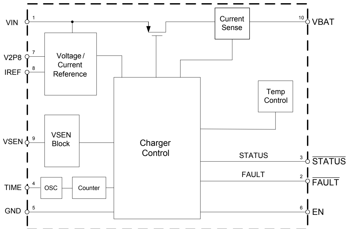
Figure 3. Functional Block Diagram of AUR9801C
