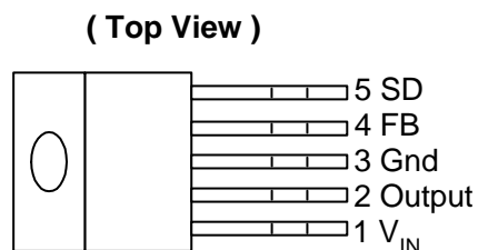
TO220-5L/TO220-5L(R)
