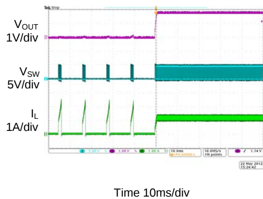
Figure 19. Short Circuit Protection Recovery ( I_{OUT}=1.2A )
