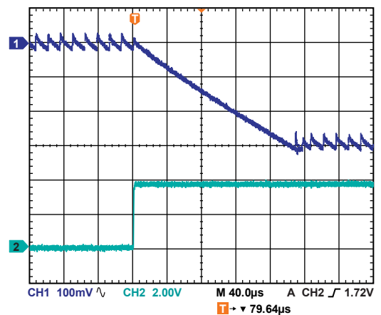
Figure 30. VSEL Change Triggering V_{OUT} Transition from 1.275 V to 0.981 V, I_{LOAD} = 10\text{ mA}
