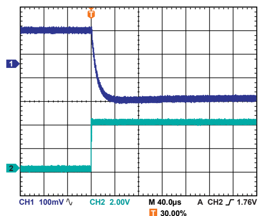
Figure 32. VSEL Change Triggering V_{OUT} Transition from 1.275 V to 0.981 V, I_{LOAD} = 200\text{ mA}
