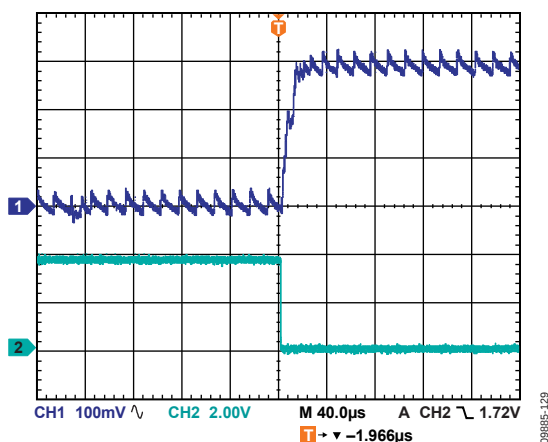
Figure 29. VSEL Change Triggering V_{OUT} Transition from 0.981 V to 1.275 V, I_{LOAD} = 10\text{ mA}
