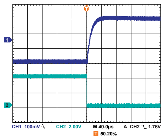
Figure 31. VSEL Change Triggering V_{OUT} Transition from 0.981 V to 1.275 V, I_{LOAD} = 200\text{ mA}
