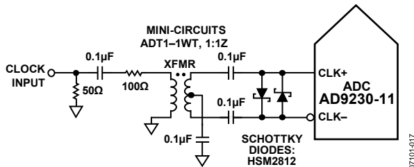
Figure 24. Transformer-Coupled Differential Clock
