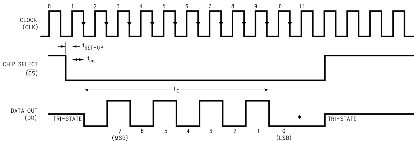
Figure 20. ADC08831 Timing
