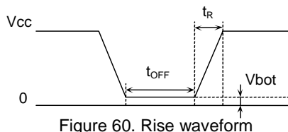
Figure 60. Rise waveform
