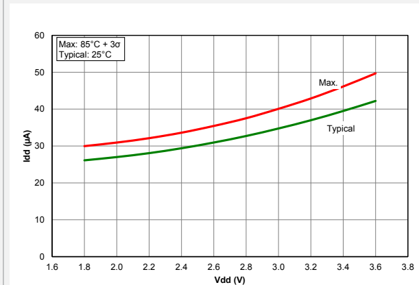
Figure 39-63. I_{PD} , Fixed Voltage Reference (FVR), PIC18LF27/47K40 only
