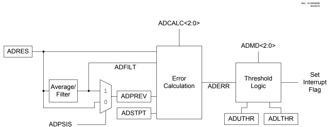
Figure 31-11. Computational Features Simplified Block Diagram
