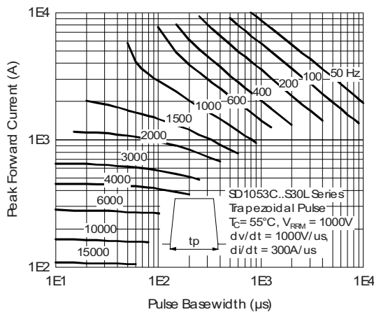
Fig. 37 - Frequency Characteristics
