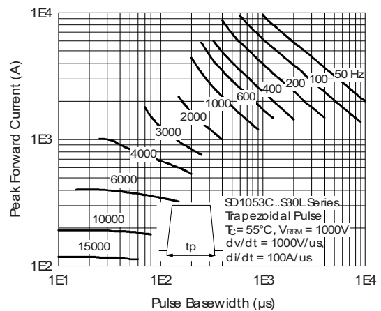
Fig. 39 - Frequency Characteristics
