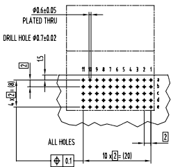
BOARD HOLE PATTERN (COMPONENT MOUNTING SIDE)
