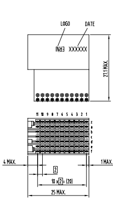
BOARD HOLE PATTERN (COMPONENT MOUNTING SIDE)
