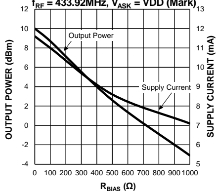
Output Power and Supply Current
