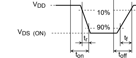
(c) V_{OUT}
