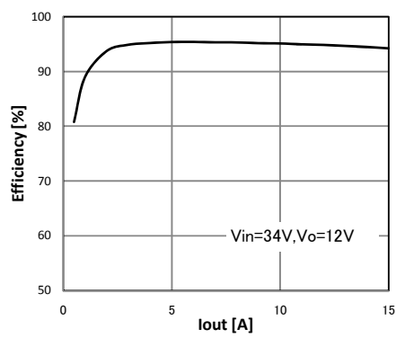
Fig.21 Efficiency
