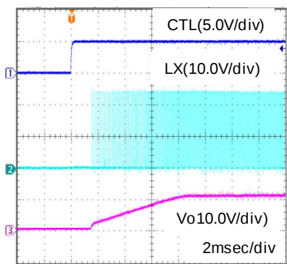
Fig.23 Start-up
