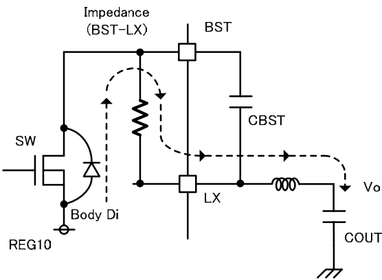
Fig.32 Current pass at PRE-BIAS and low setting output voltage
