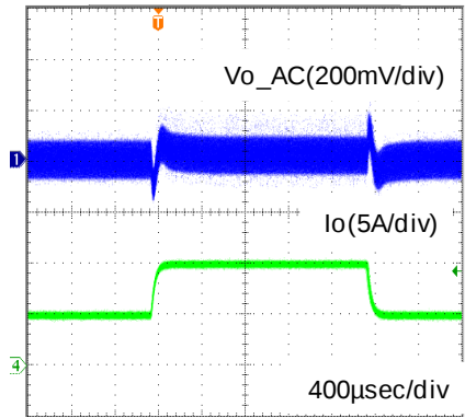
Fig.22 Load Response(Io=5A↔10A)
