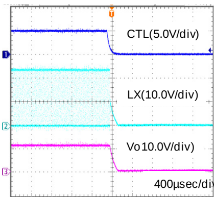
Fig.25 Stop (Rload=2.5Ω)
