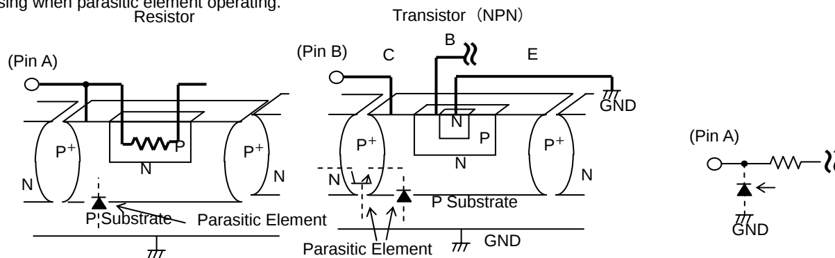
Fig.41 Example of simple structure of Bipolar IC
