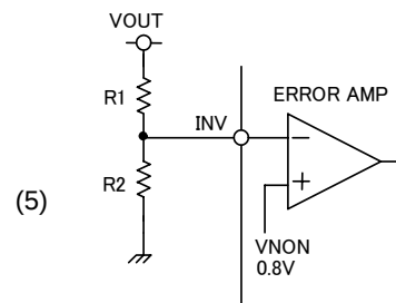
Fig.37 Vout setting
