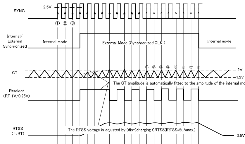
Fig.28 timing chart about External Mode
