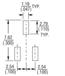
RECOMMENDED PCB LAYOUT - "W" & "X"
