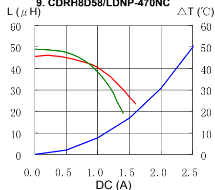
9. CDRH8D58/LDNP-470NC
