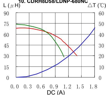
10. CDRH8D58/LDNP-680NC
