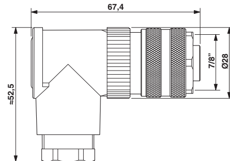
Dimensioned drawing
