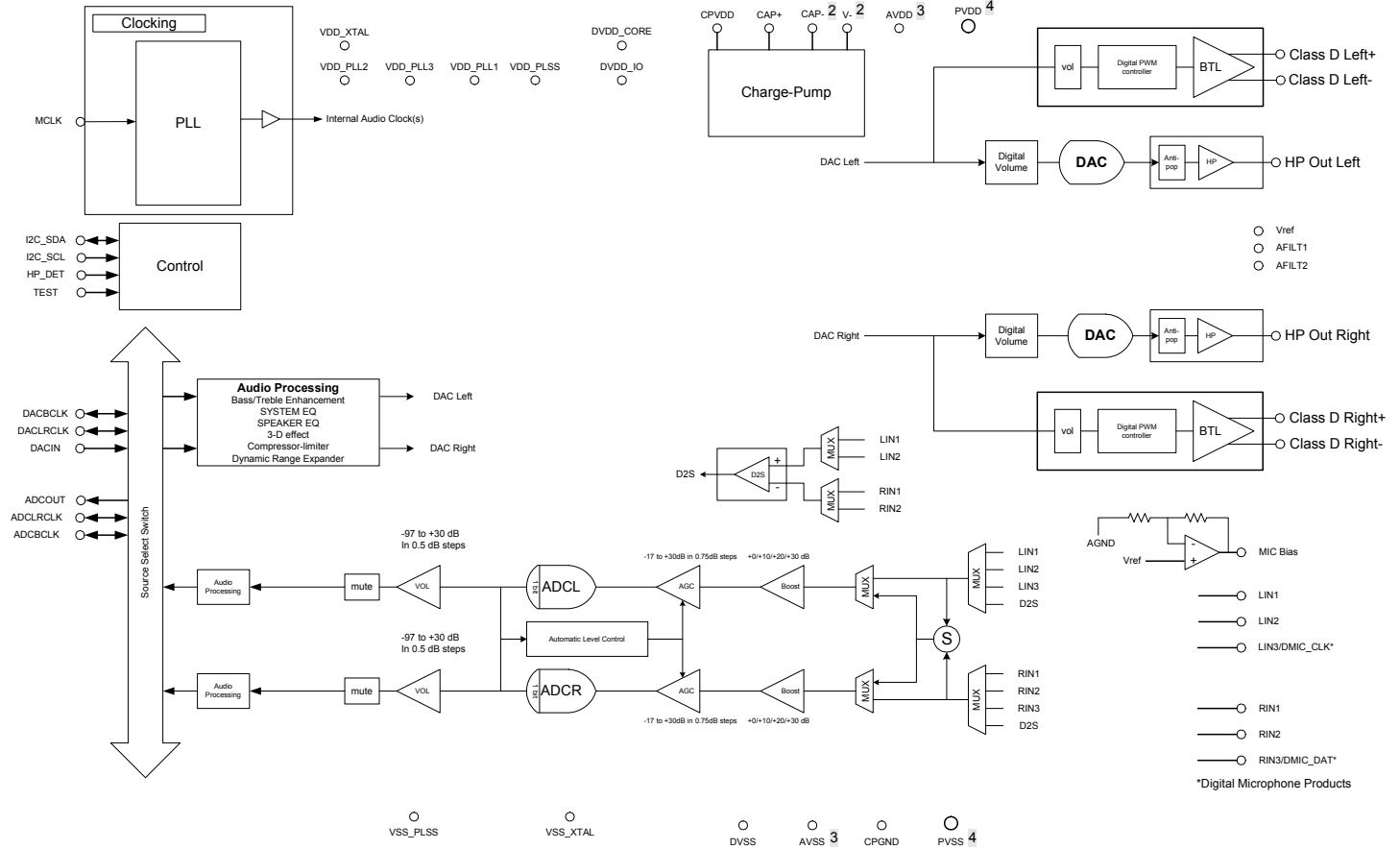
Figure 1. ACS422x68 TLA Block Diagram
