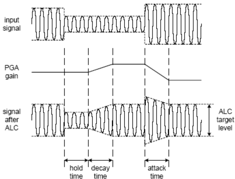
Figure 21. ALC Operation
