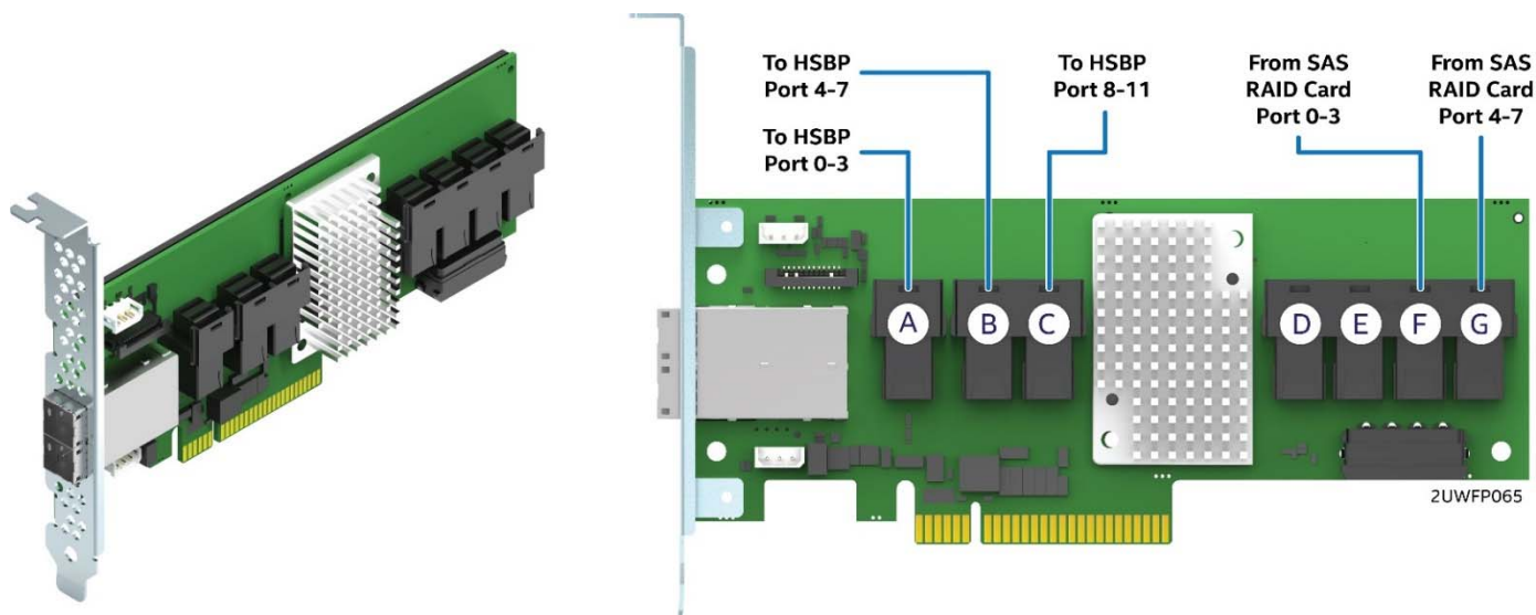
Figure 75. Intel® RAID Expander RES3FV288 connector identification
