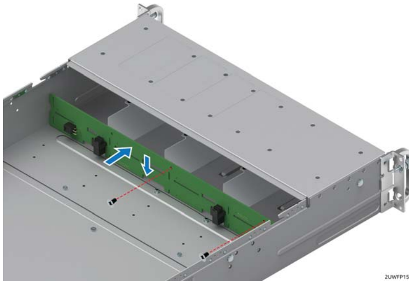
Figure 47. 3.5" backplane placement
