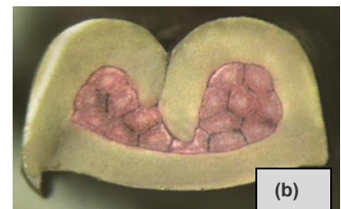
Significant flash can be generated with excessive anvil to crimper clearance, as shown by nominal design condition (a) and +0.003 in over nominal condition (b)
