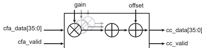
Figure 51-22. CC Block Diagram
