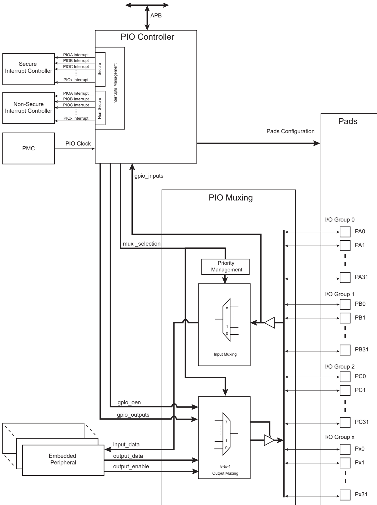
Figure 33-1. Block Diagram
