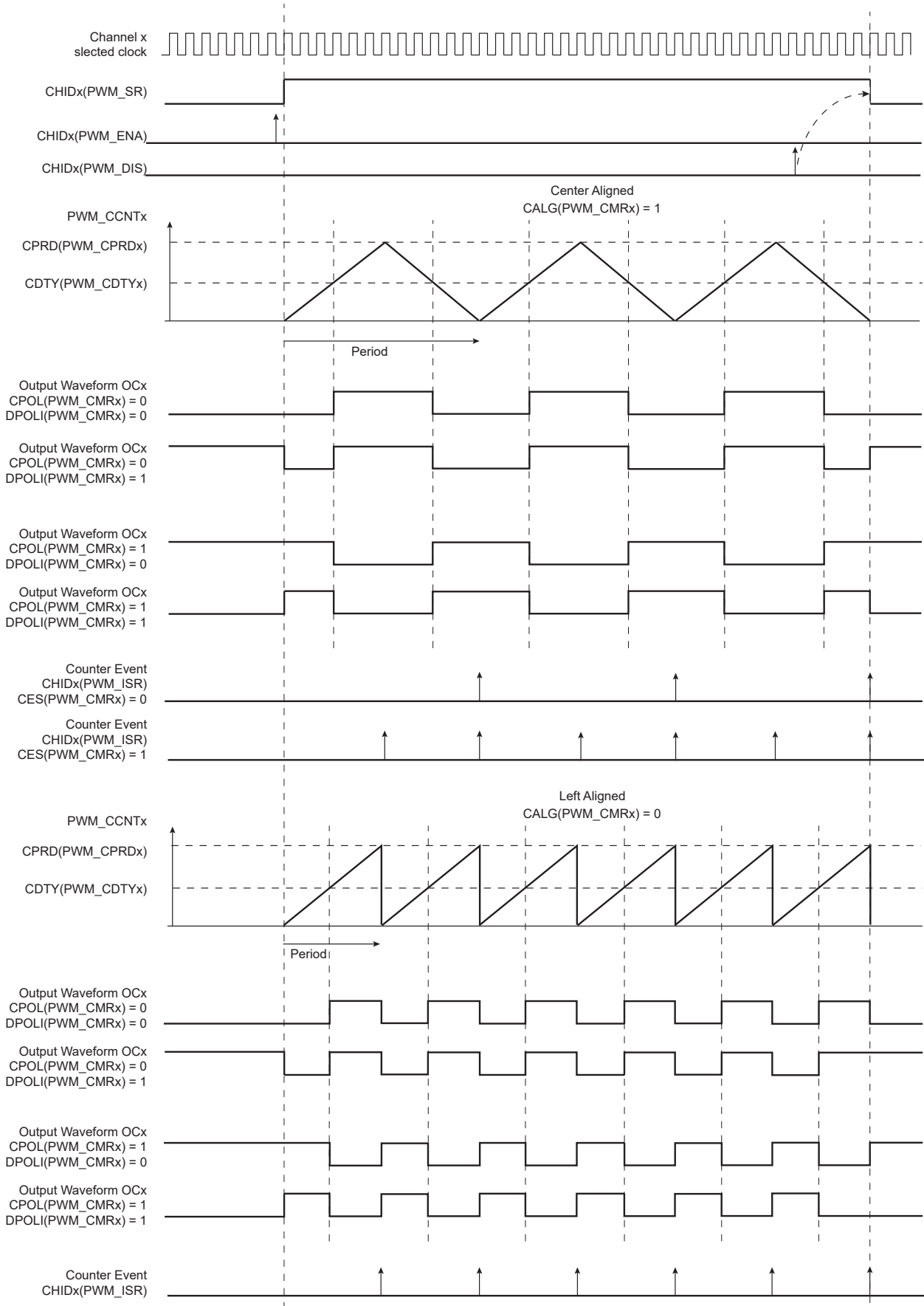
Figure 55-5. Waveform Properties
