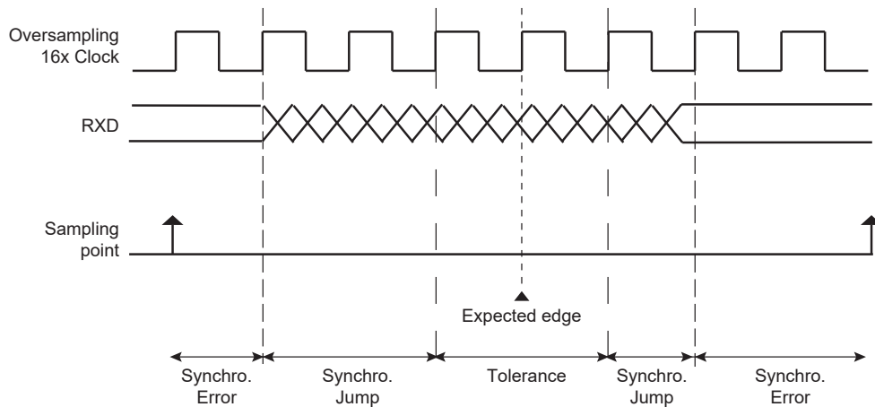
Figure 46-10. Bit Resynchronization
