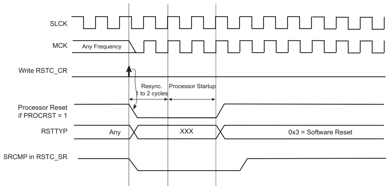
Figure 23-6. Software Reset
