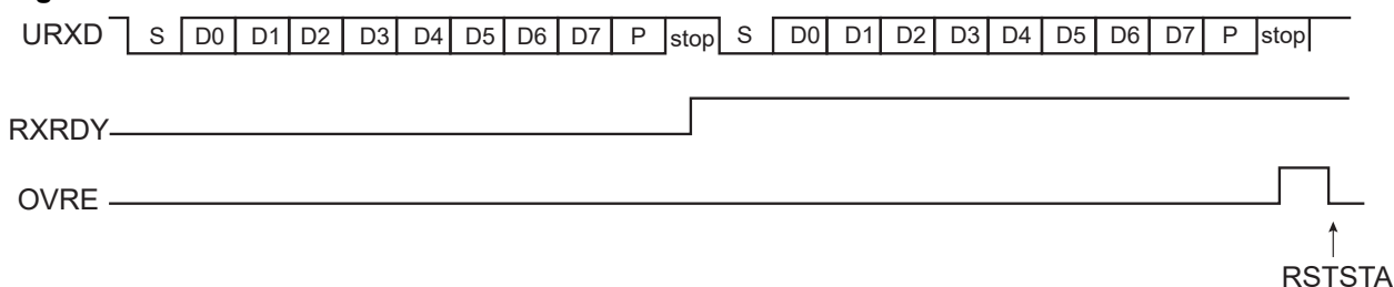
Figure 47-3. Start Bit Detection
