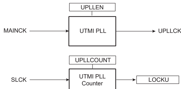
Figure 31-6. UTMI PLL Block Diagram
