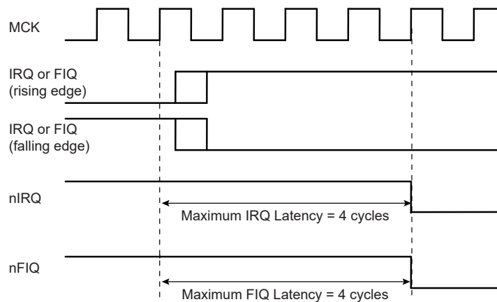
Figure 21-6. External Interrupt Edge Triggerged Source
