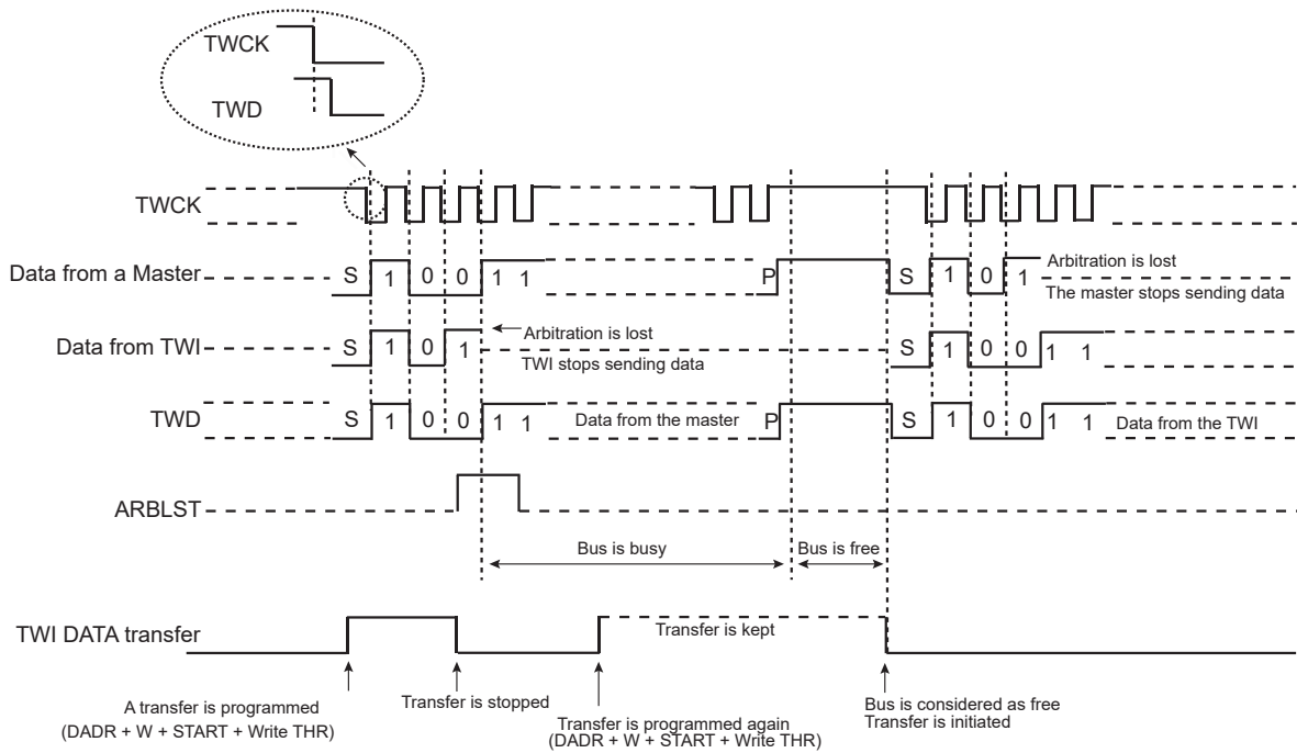
Figure 46-110. Arbitration Cases
