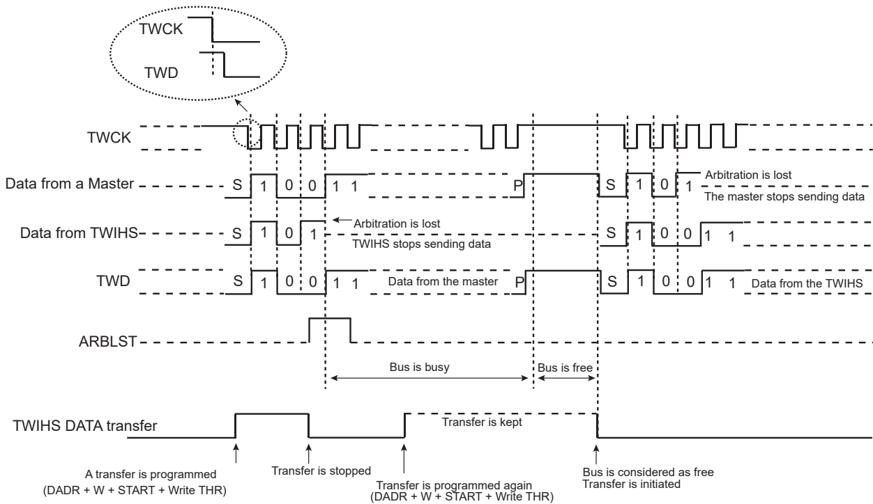
Figure 45-29. Arbitration Cases
