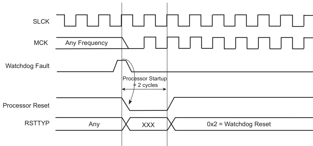
Figure 23-7. Watchdog Reset
