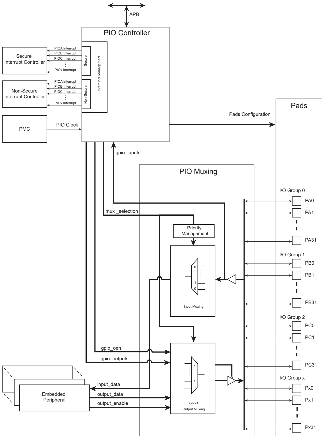
Figure 33-1. Block Diagram
