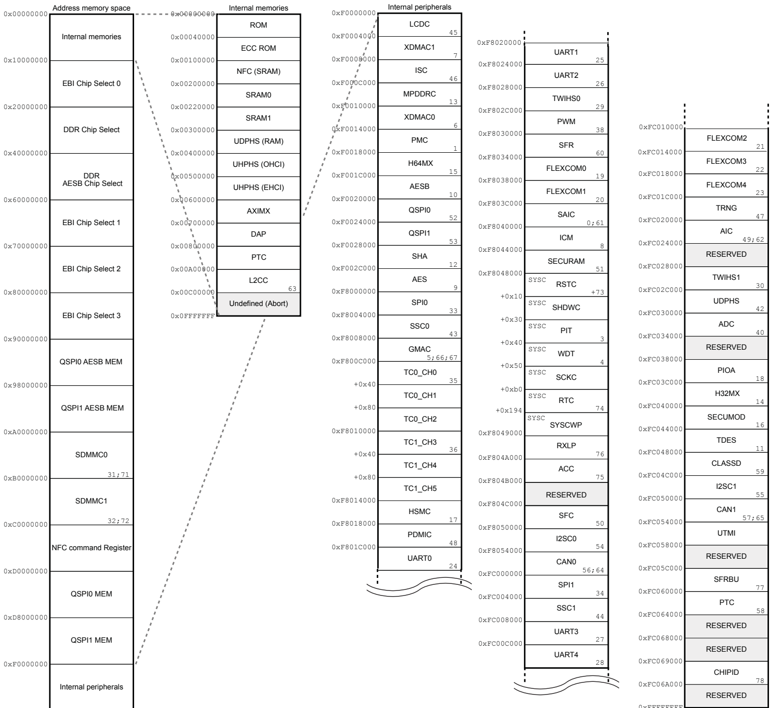
Figure 8-1. Memory Mapping
