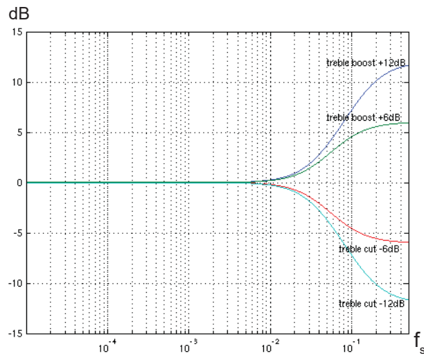
Figure 42-7. Treble Filters Response
