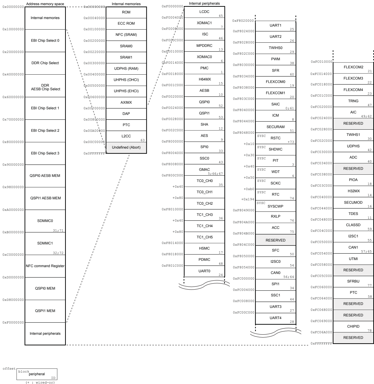
Figure 8-1. Memory Mapping
