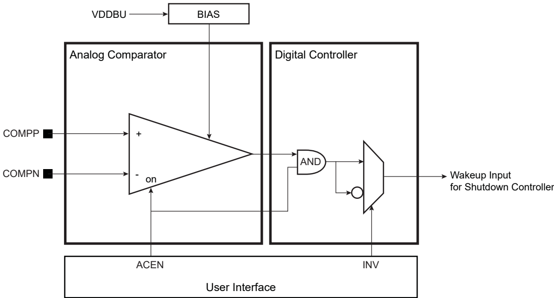
Figure 63-1. Analog Comparator Controller Block Diagram
