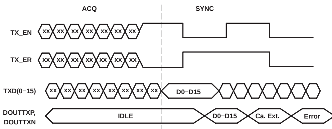
Figure 7. Transmit Side Timing Diagram
