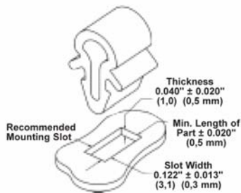
MOUNTING INFORMATION
