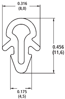
PROFILE DIMENSION
