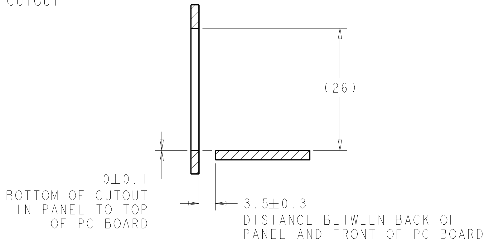
SECTION U-U
