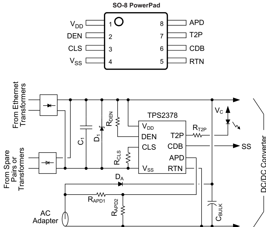
Figure 1. Typical Application
