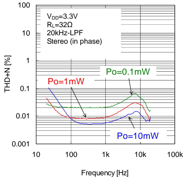
Figure 18. THD+N vs Frequency ( V_{DD} = 3.3\text{V} , R_L = 32\Omega )
