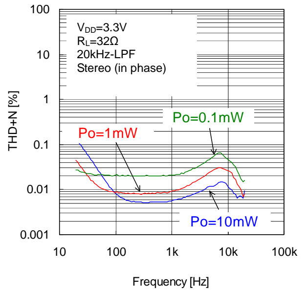
Figure 18. THD+N vs Frequency ( V_{DD}=3.3V , R_L=32\Omega )
