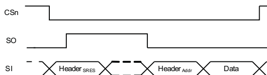
Figure 3-7. SRES Command Strobe
