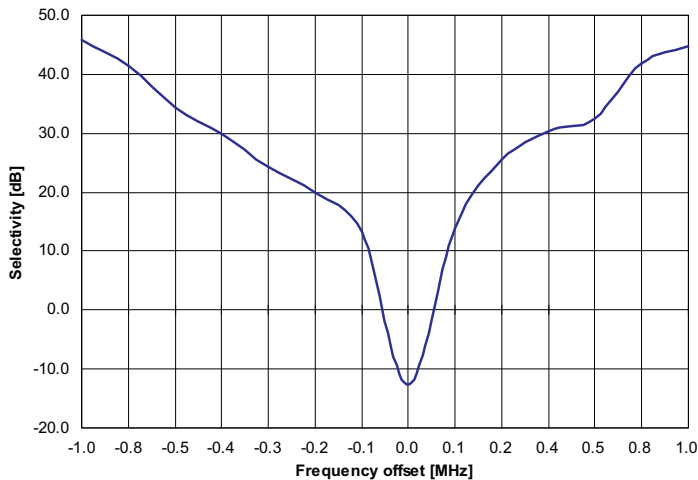
Figure 2-2. Typical Selectivity at 38.4-kBaud Data Rate, 868 MHz, GFSK, 20-kHz Deviation, IF Frequency 152.3 kHz, Digital Channel Filter Bandwidth 100 kHz
