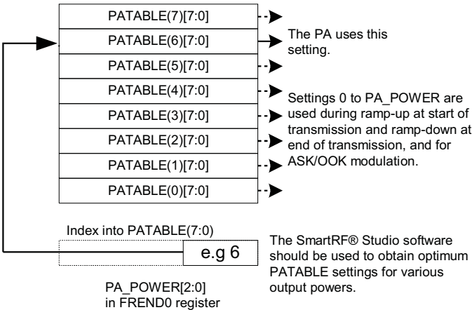
Figure 3-21. PA_POWER and PATABLE
