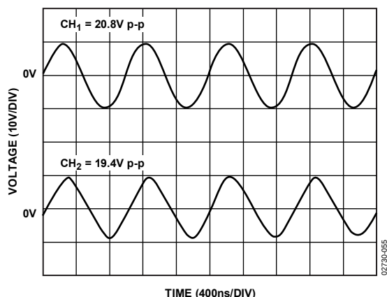
Figure 55. AD8610 FPBW
