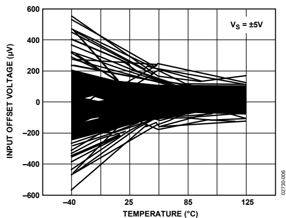
Figure 6. Input Offset Voltage vs. Temperature at \pm 5V (300 Amplifiers)
