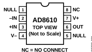
Figure 1. 8-Lead MSOP and 8-Lead SOIC_N
