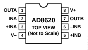
Figure 2. 8-Lead SOIC_N
