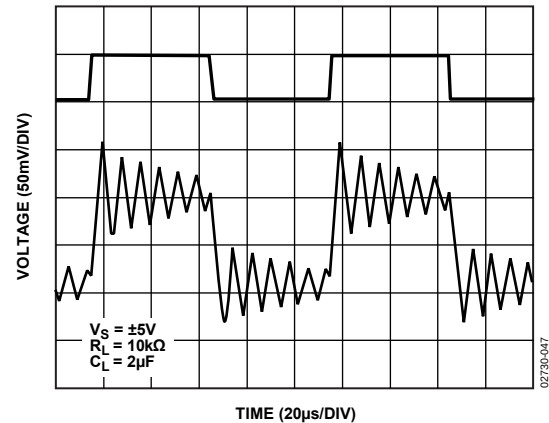
Figure 47. OPA627 Capacitive Load Drive, A_V = +2
