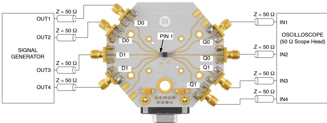
Figure 5. Lab Setup
