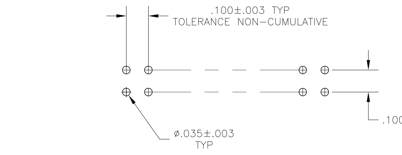
RECOMMENDED HOLE LAYOUT
