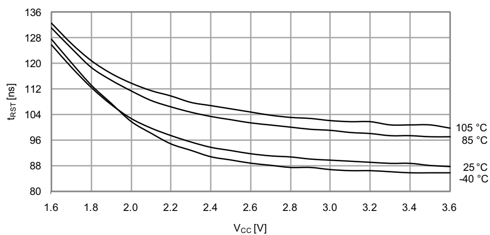
Figure 36-48.Minimum Reset Pin Pulse Width vs. V_{CC}
