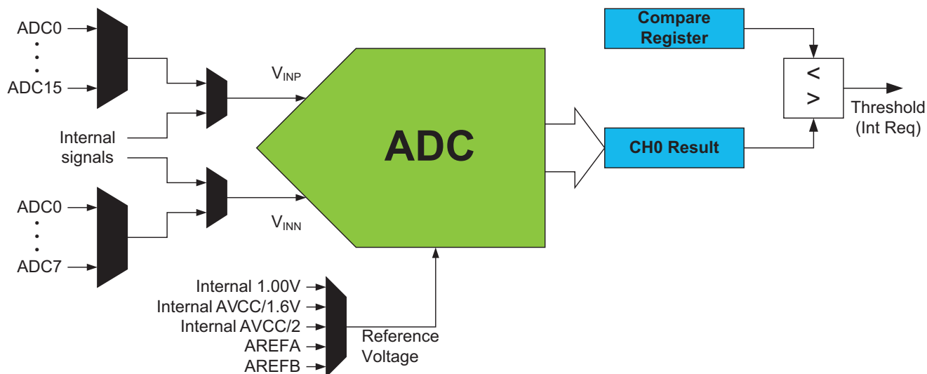
Figure 28-1. ADC Overview
