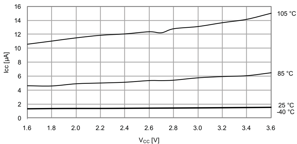
Figure 36-16. Power-down Mode Supply Current vs. V_{CC}
