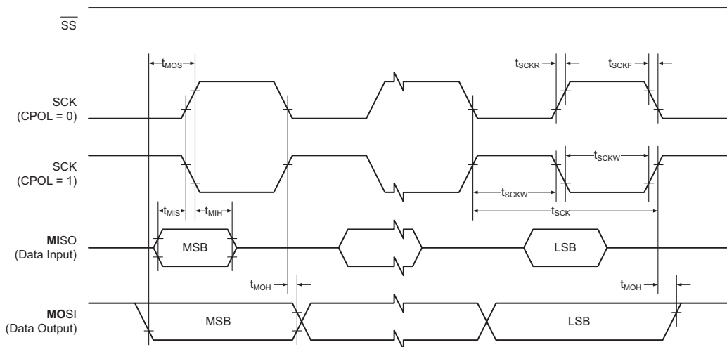
Figure 35-5. SPI Timing Requirements in Master Mode
