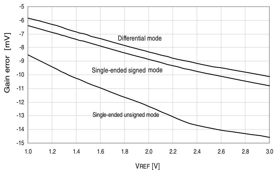
Figure 36-36.Gain Error vs. V_{REF} T = 25^{\circ}\text{C} , V_{CC} = 3.6\text{V} , ADC sample rate = 300ksps
