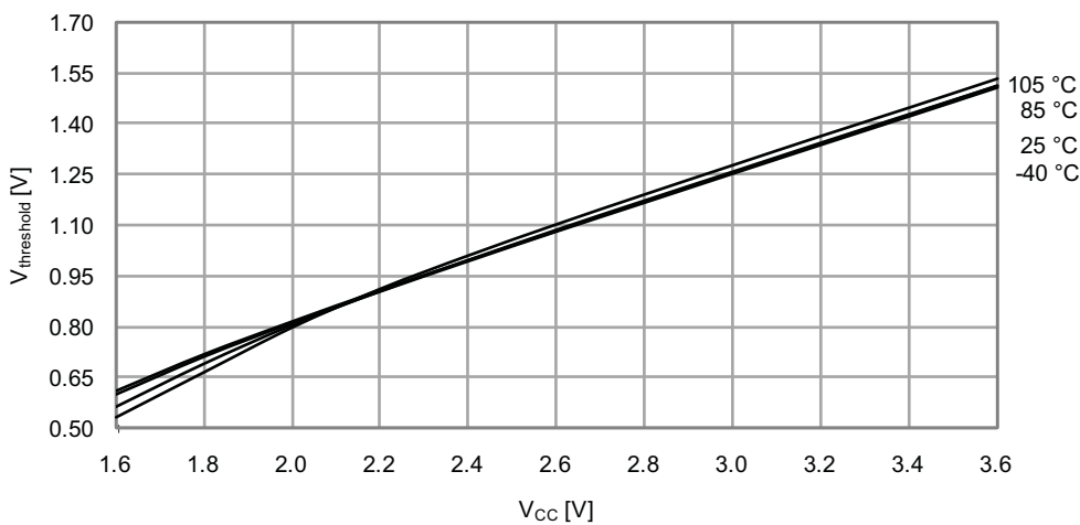
Figure 36-28. I/O Pin Input Threshold Voltage vs. V_{CC} V_{IL} I/O pin read as “0”
