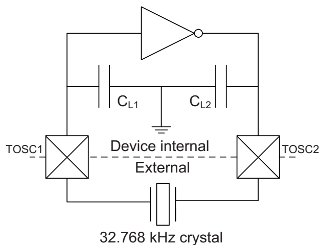
Figure 35-4. TOSC Input Capacitance
